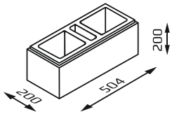
BH20, RP20, RD20 Pfeilerblock / Mauerblock
